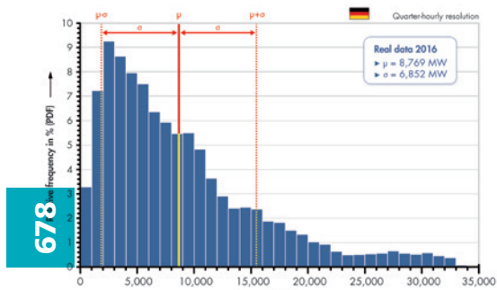
Frequency distribution of electric power output of the German wind fleet in 2016.
