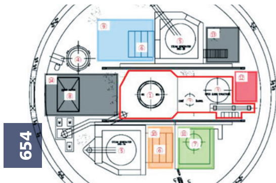
Reactor Building Layout in Kori unit 1.
