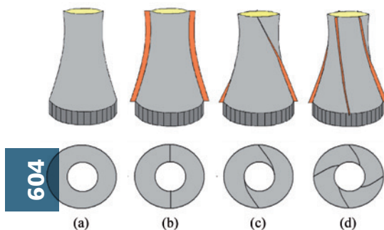
Schematically views of usual and finned type cooling towers.
