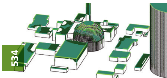
Simulation results for the assessment of lightning effect on a nuclear plant.
