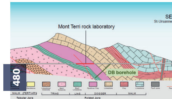
Vertical section of the Mont Terri.
