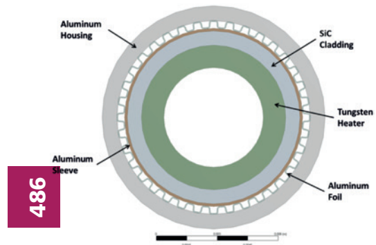
Schematic showing the general design concept for the SiC cladding irradiation.
