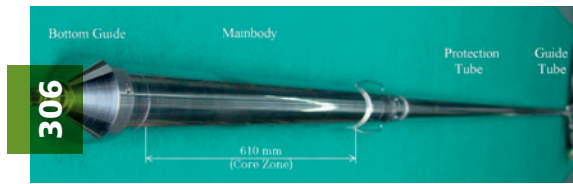
| Instrumented capsule for the material irradiation test.
