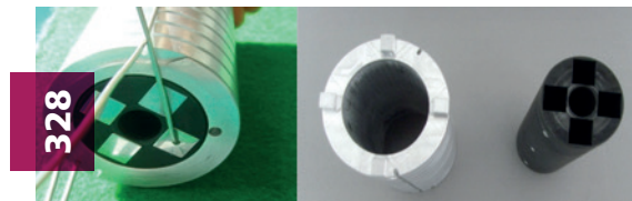
| Structure of double thermal media.
