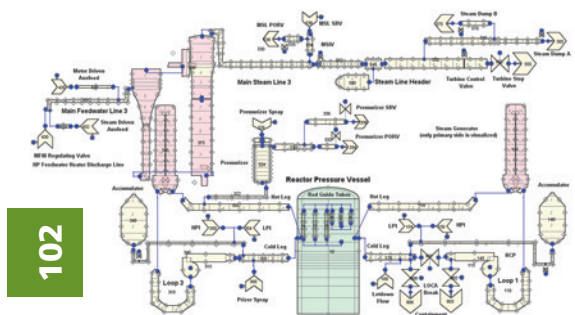
SNAP view of the 3-loop PWR TRACE model.
