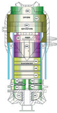
Nodalization for RCS in RETRAN.
